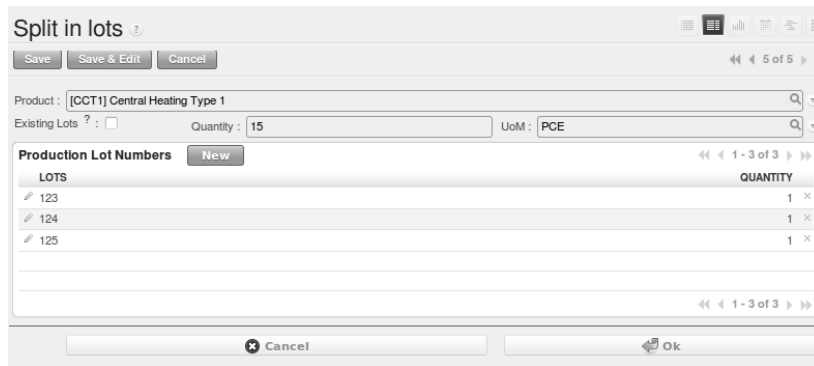
Figure 6.43: Splitting a Lot into uniquely Identified Parts
