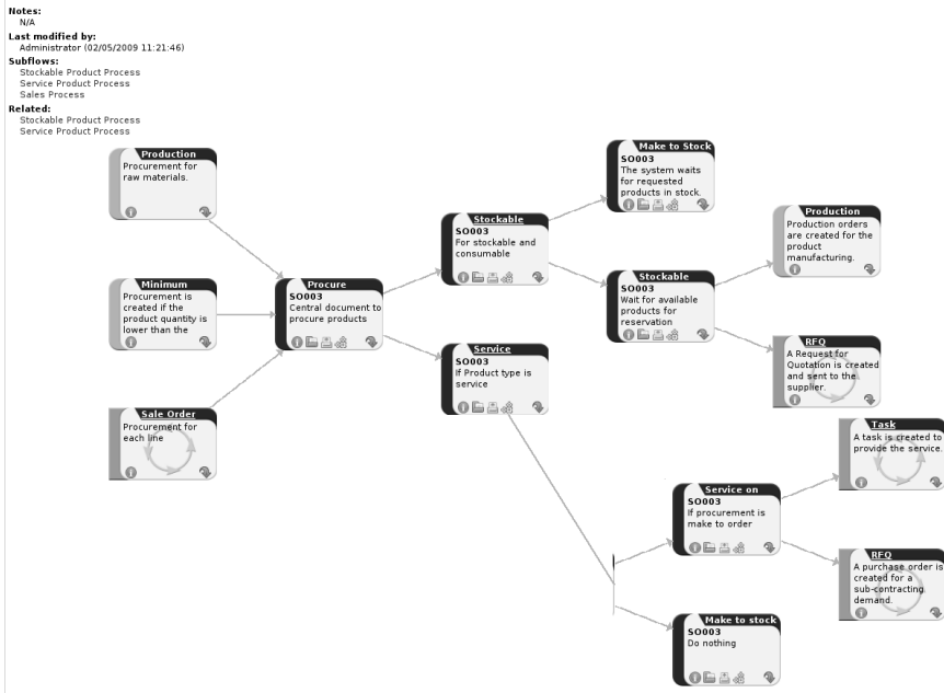
Figure 6.30: Workflow for Automatic Procurement, depending on the Product Configuration
