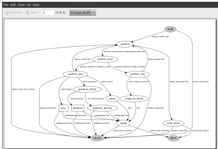
Figure 6.36: Workflow for Handling a Procurement according to Product Configuration
